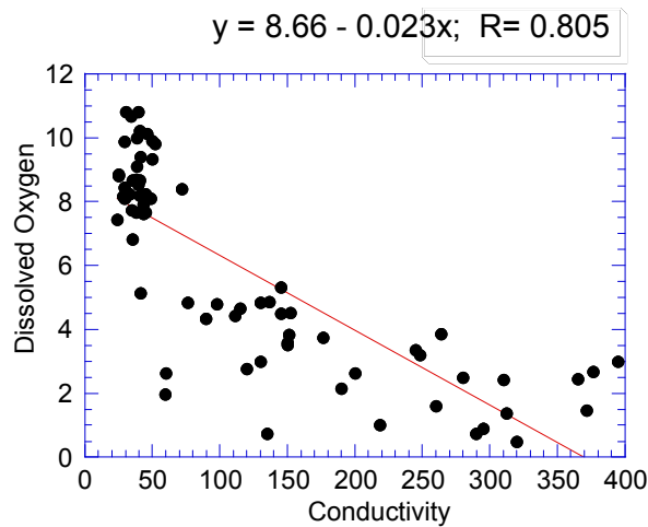
Fig.3: Overall relationship between electrical conductivity ( \mu\text{S}/\text{cm} ) and dissolved oxygen ( \text{mg}/\text{L} ) from the upstream to the downstream of the Langat River.
